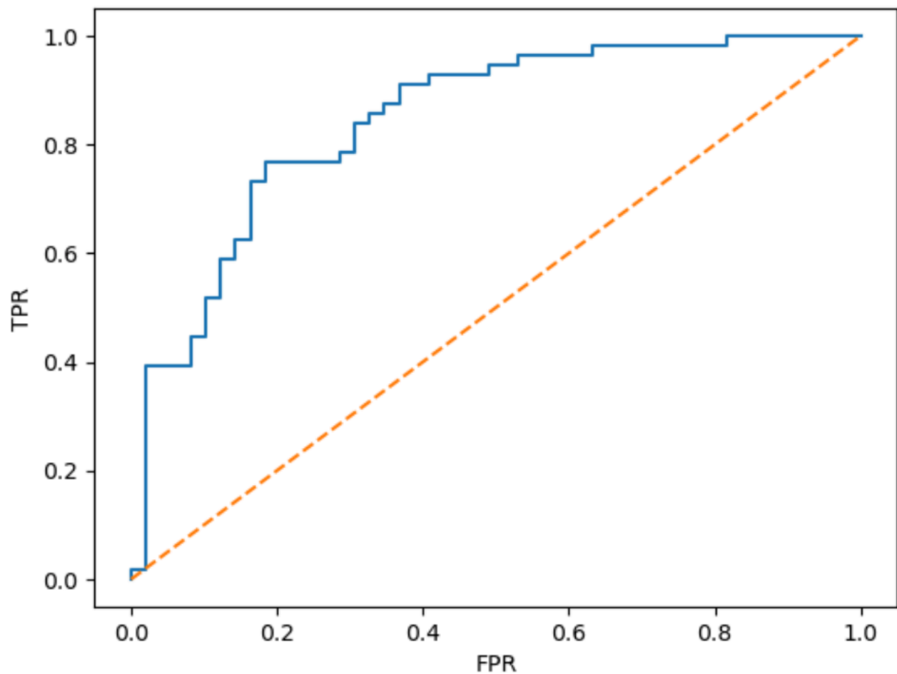
ROC Curve - XGBoost
